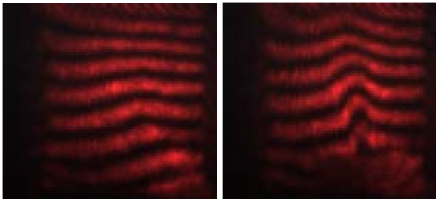
Helium Jet Horizontal fringes
