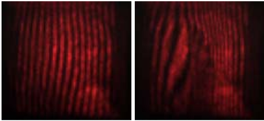
Soldering Iron Vertical fringes
