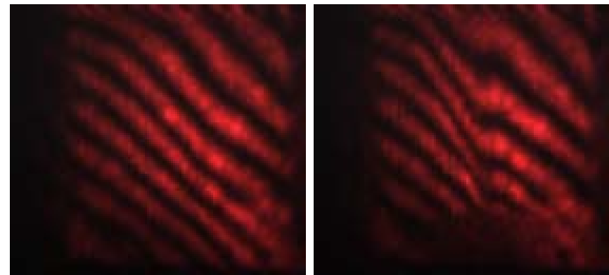
Helium Jet Slant fringes
